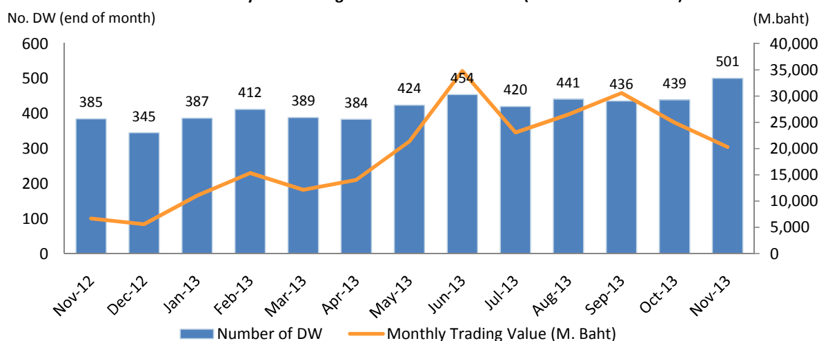
Monthly DW Trading Value vs Number of DW (Nov 2012 - Nov 2013)
