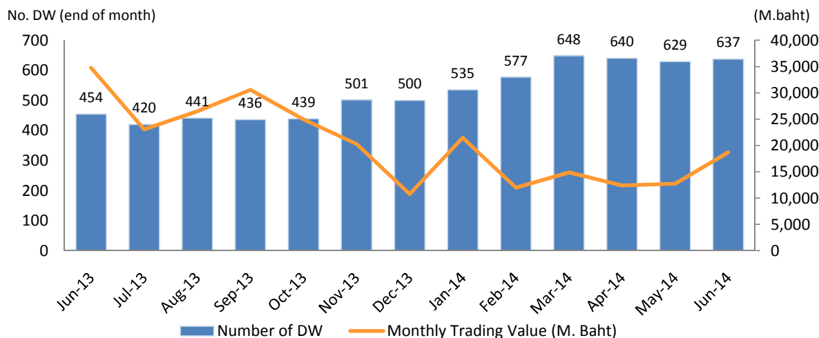
Monthly DW Trading Value vs Number of DW (Jun 2013 - Jun 2014)
