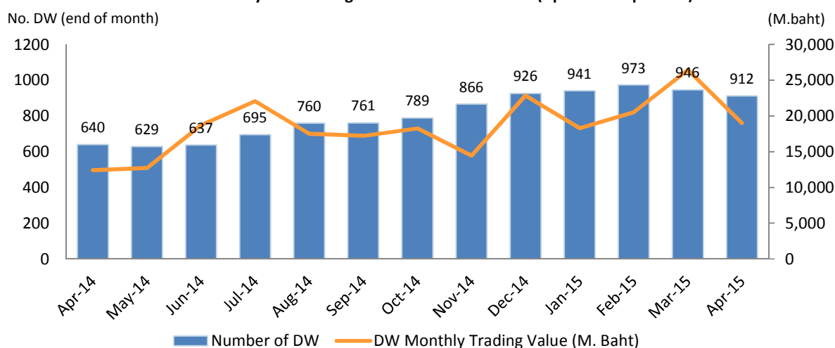
Monthly DW Trading Value vs Number of DW (Apr 2014 - Apr 2015)
